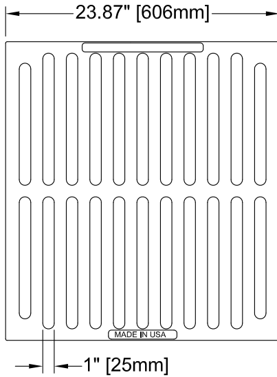
GRATE TOP VIEW (ROTATED 90°)
