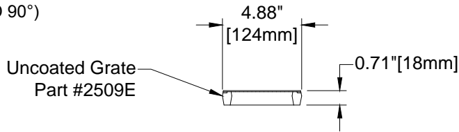
GRATE END VIEW
