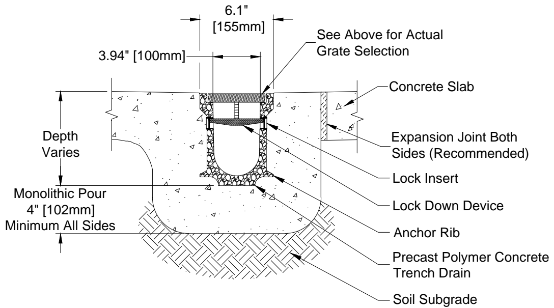
END CROSS SECTION VIEW
